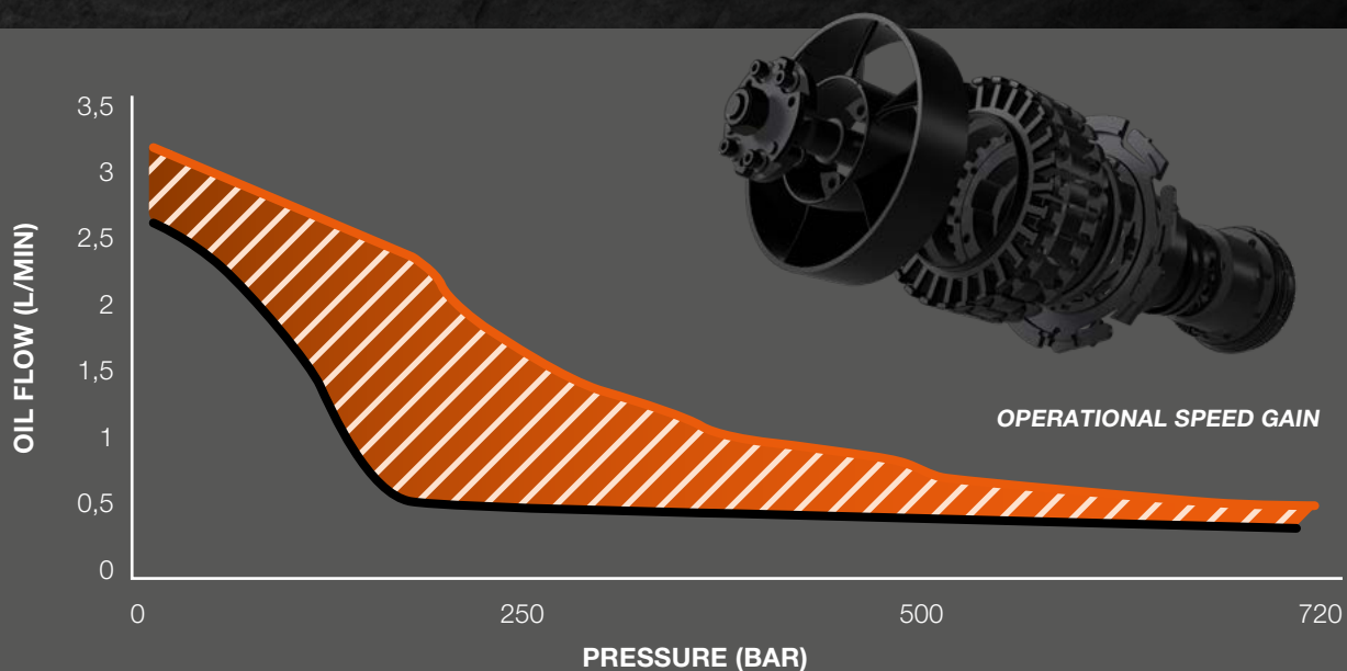
Oil Flow vs. pressure: The Apeiron® vs. main competition
